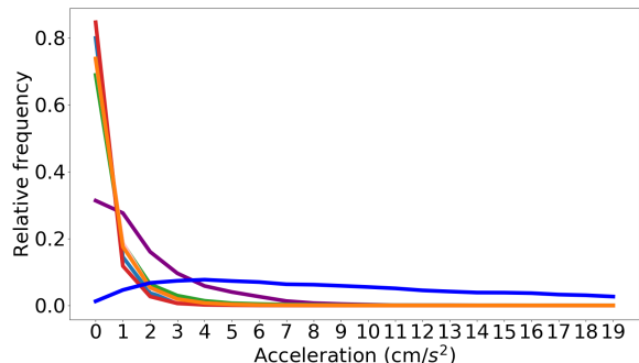
(b) Acceleration histogram for shoulders. Legend as in (a).
