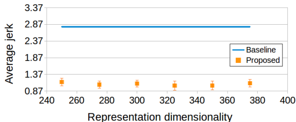
(b) Average jerk. Baseline jerk is 2.8 \pm 0.3 while ground-truth jerk is 0.54.
